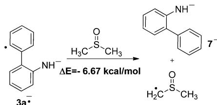
Scheme 10. ET from 6a^{\bullet-} to 3a^-
