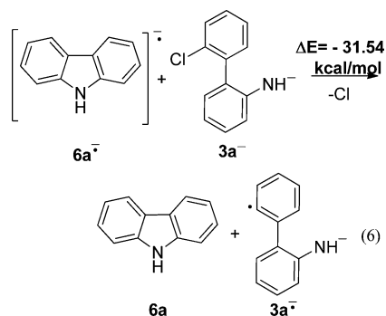
Scheme 10. ET from 6a^{\bullet-} to 3a^-
