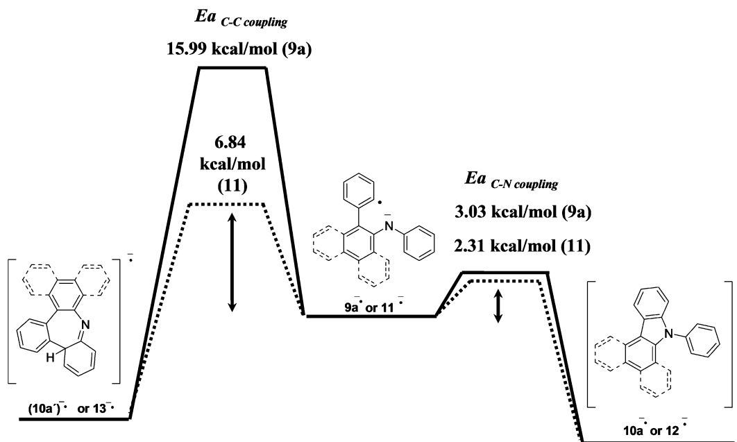
Scheme 12. Evaluation of C–N vs C–C Cyclization for 9a^{\bullet-} and 11^{\bullet-} by ET
