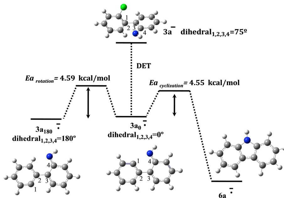
Scheme 9. Hydrogen Abstraction by 3a^{\bullet-} from the Solvent
